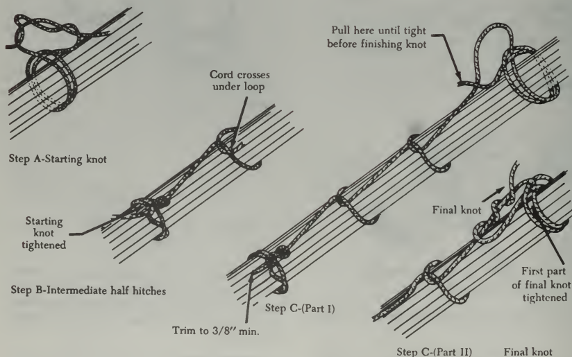
FIGURE 4-100. Single-cord lacing.
